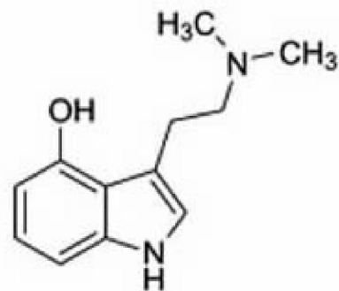
Psilocin
