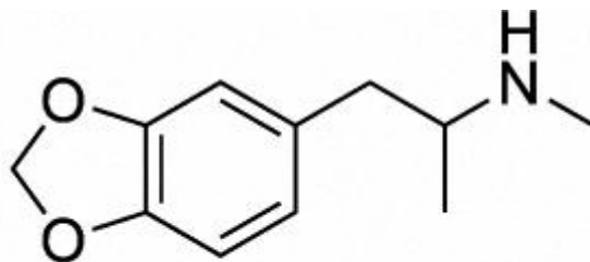
MDMA
