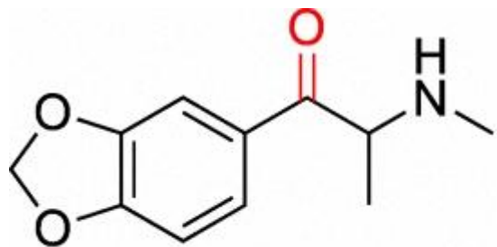
Methylone
