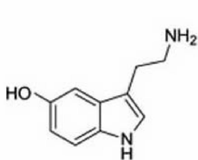
Serotonin
