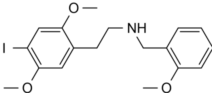
25I-NBOMe = 4-iodo-2,5-dimethoxy-N-(2-methoxybenzyl)PEA
