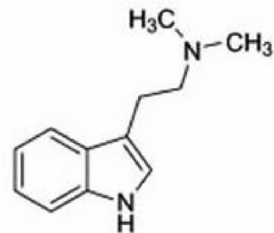
N,N-Dimethyltryptamine (DMT)
