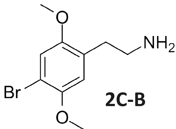
4-broom-2,5-dimethoxy-PEA
